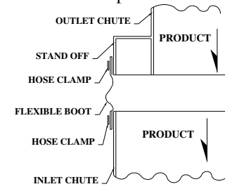
Round or elliptical boot Connection with hose clamp
